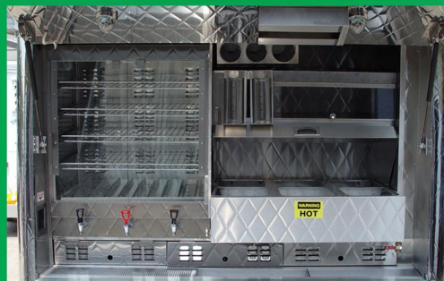
Remote coffee faucets, hot holding oven and steam table
